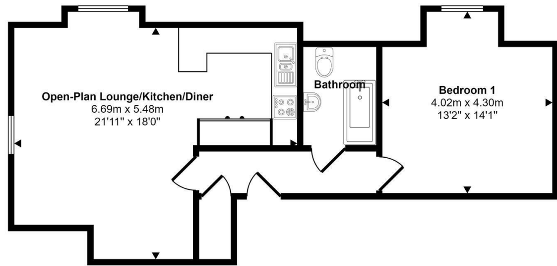
Floorplan
